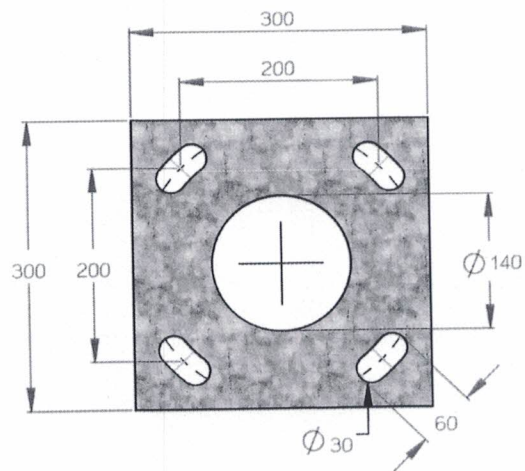
BASE PLATE DETAIL SCALE 1 : 8
