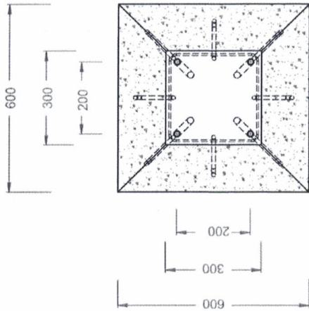
TOP VIEW SCALE 1 : 15
